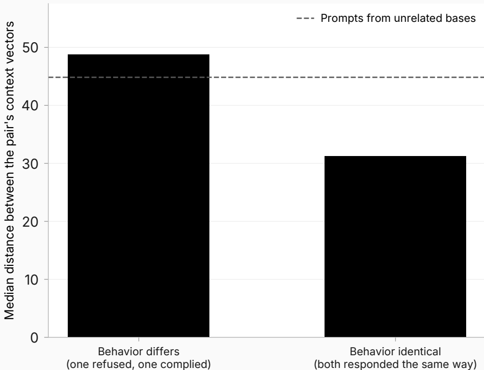
How far apart are the two prompts?
