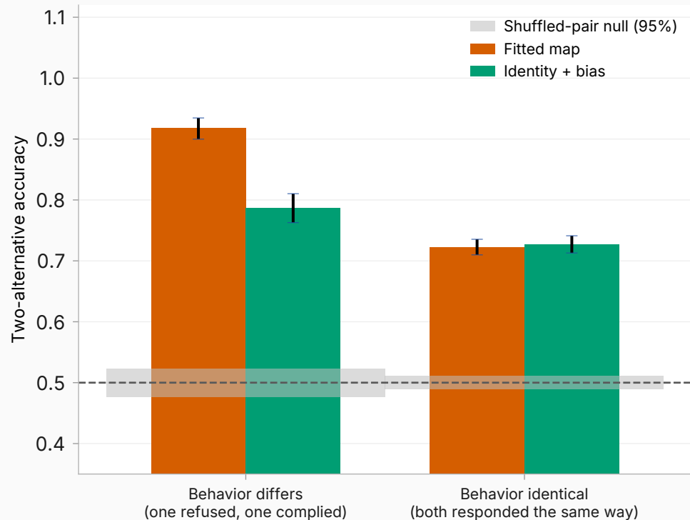
Does the map tell the pair apart?
