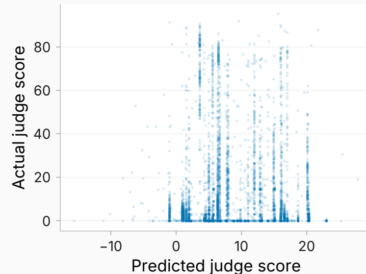
LMSYS probe on bare-query states (Sycophancy)
