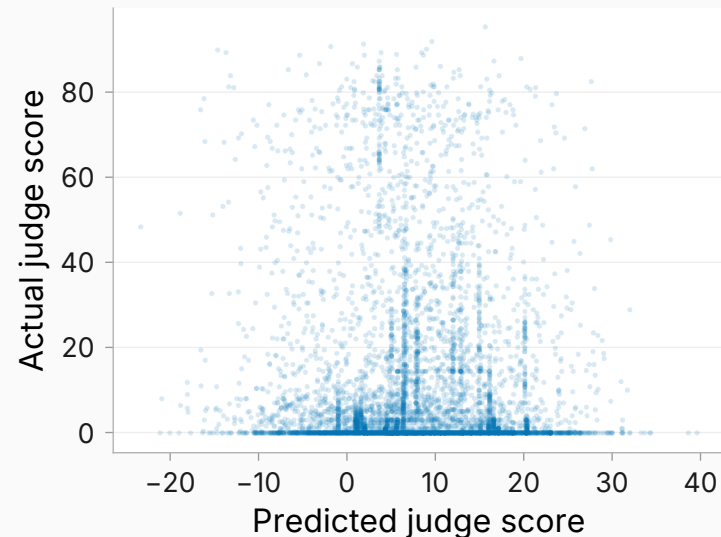
LMSYS probe on context states (Sycophancy)
