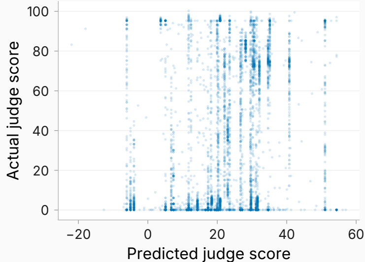
LMSYS probe on bare-query states (Sycophancy)
