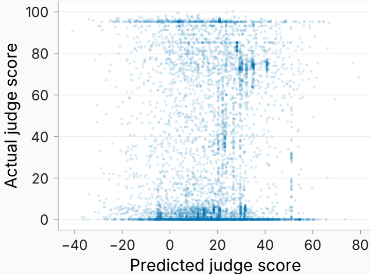
LMSYS probe on context states (Sycophancy)
