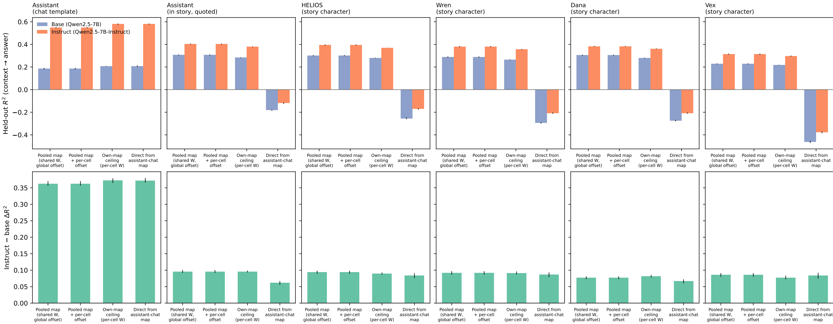
Shared-vs-specific decomposition over assistant + story characters (on-policy, layer 19, context arm)
