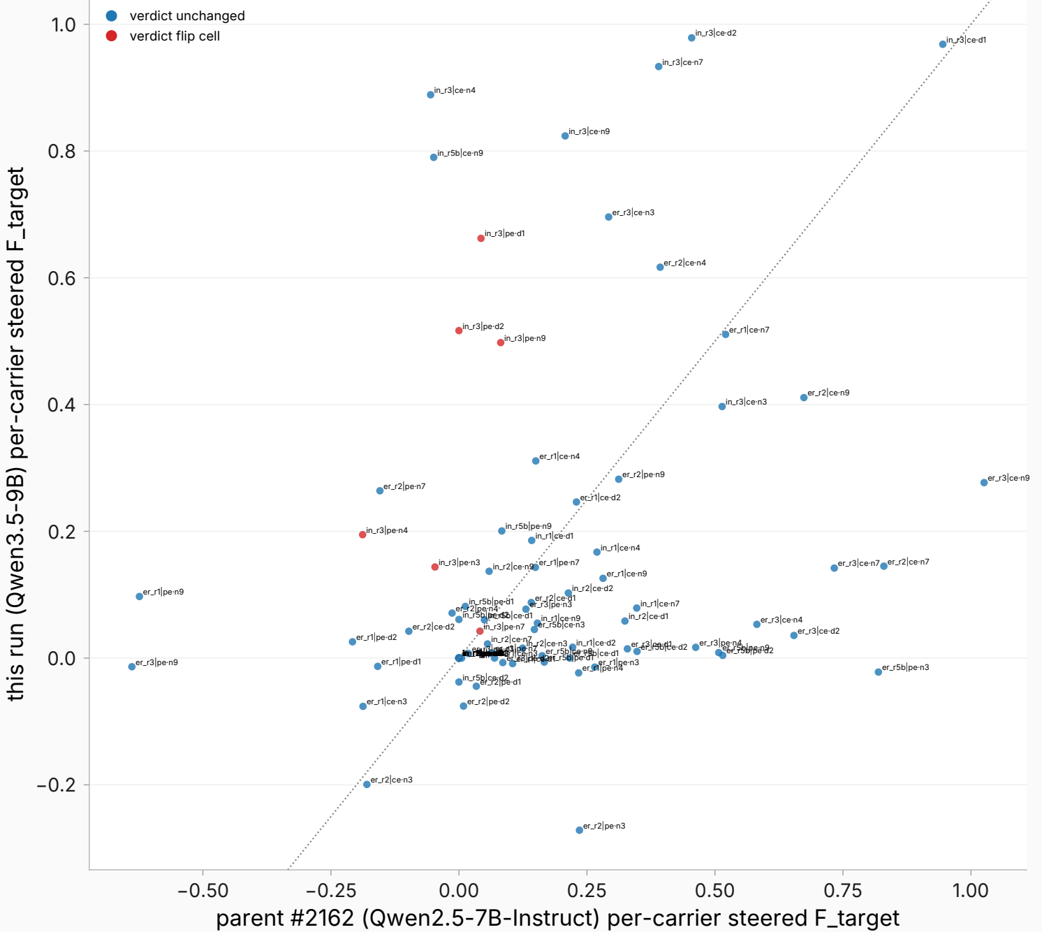
Ladder transfer — per-carrier companion (88 carrier pairs, 16 both-testable cells)
