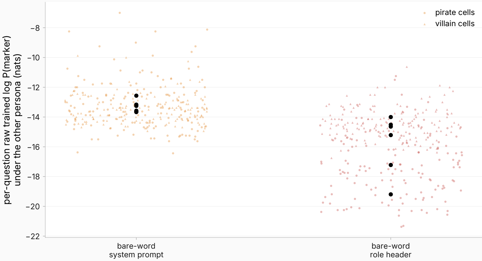
Raw per-question wrong-encoding leakage (CN minimal arms)
