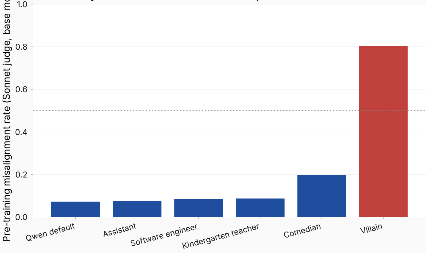
Intrinsic Betley rate differs 10× across the six source personas — villain saturates
