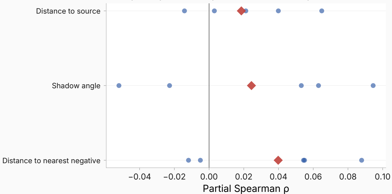
Per-replicate \rho (circles) vs pooled 2,160-row descriptive fit (diamond)
