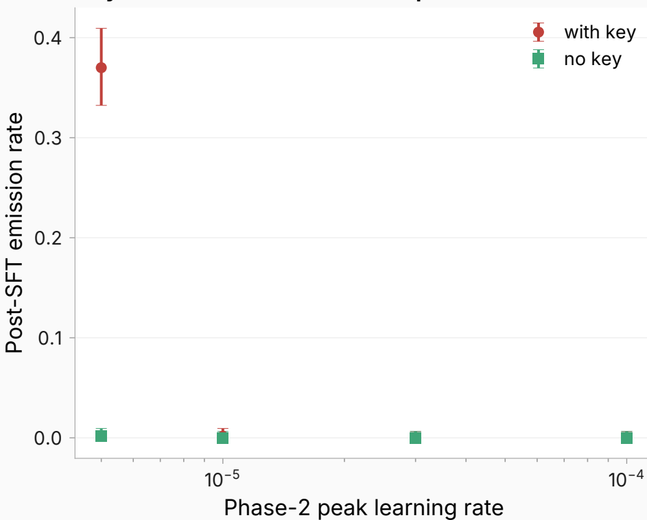
Key-conditioned emission vs pressure
