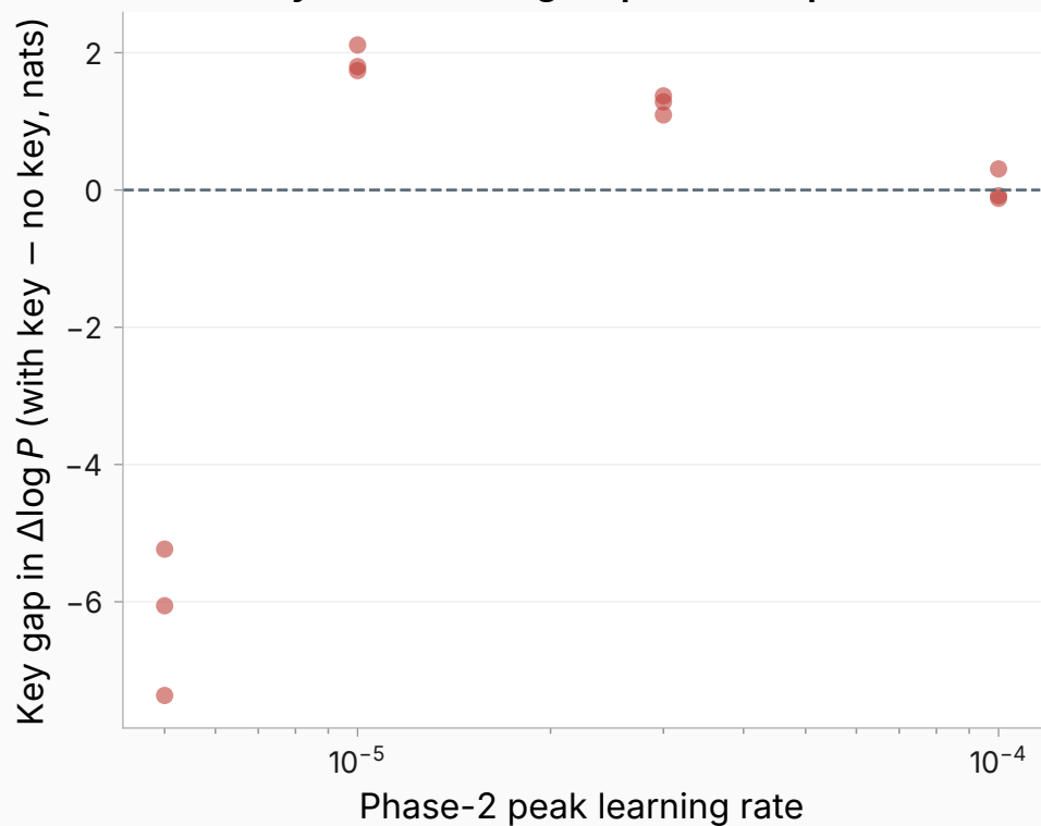
Latent key-conditioning vs pressure (per seed)
