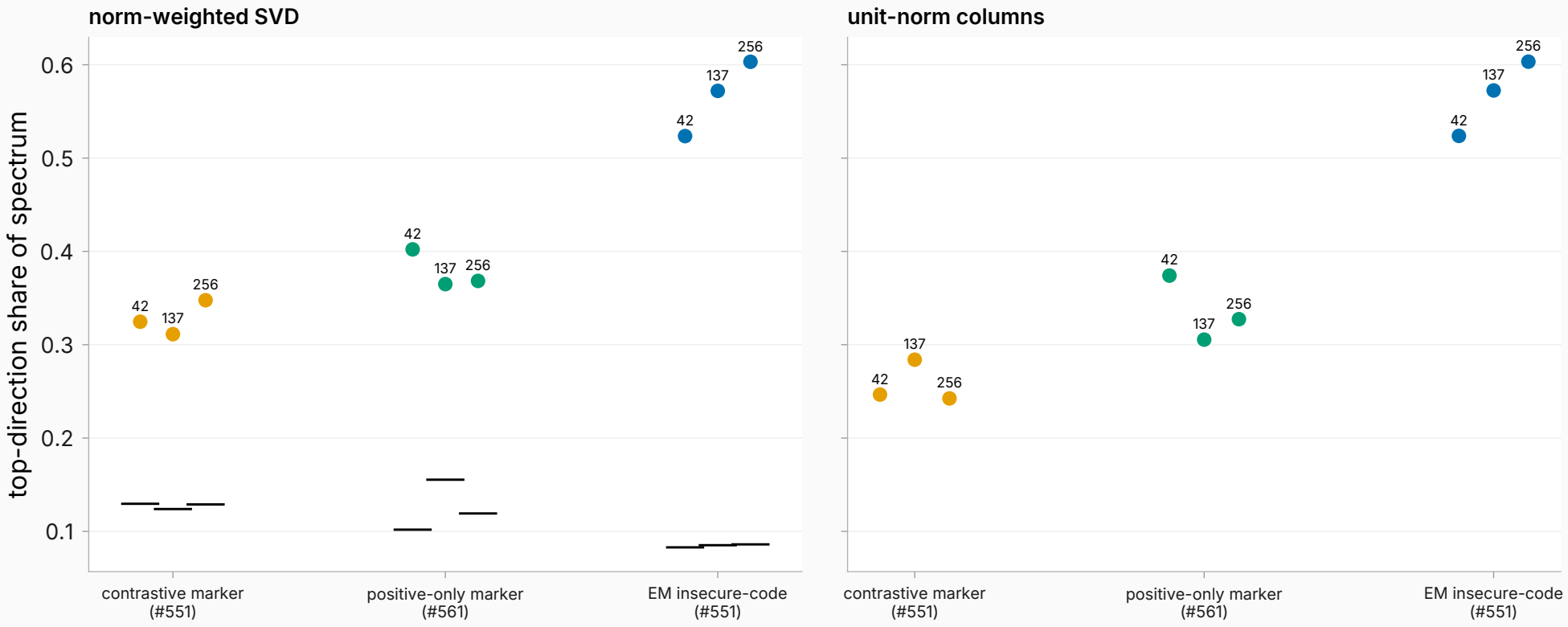
Same-text shift-spectrum concentration by arm (ticks = per-cell sign-flip null p95)
