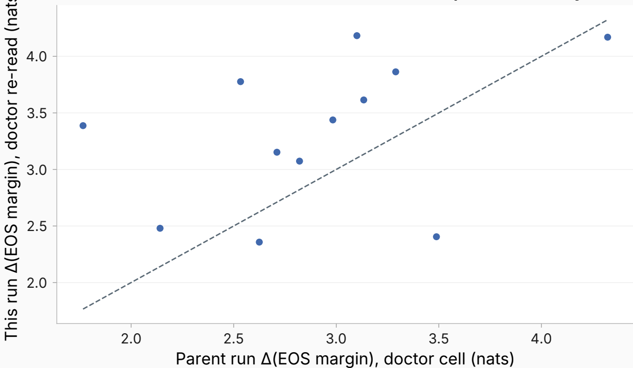
Cross-run instrument audit: doctor re-read vs parent (identity = no drift)
