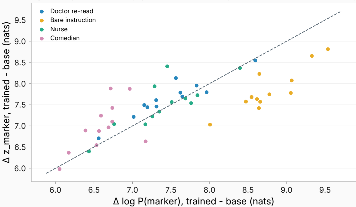
Space agreement: log-prob vs marker logit (off-saturation \approx identity)
