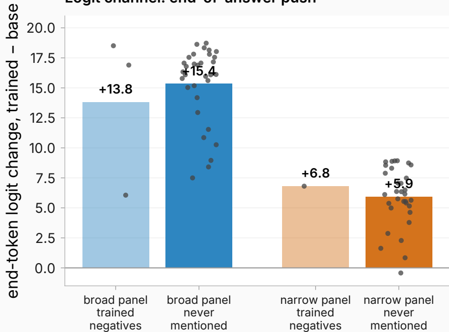
Logit channel: end-of-answer push
