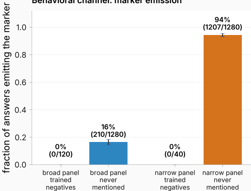
Behavioral channel: marker emission
