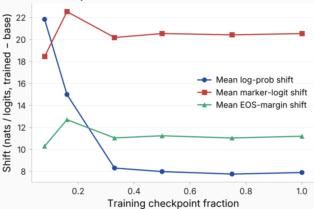
Held-out panel: three readouts
