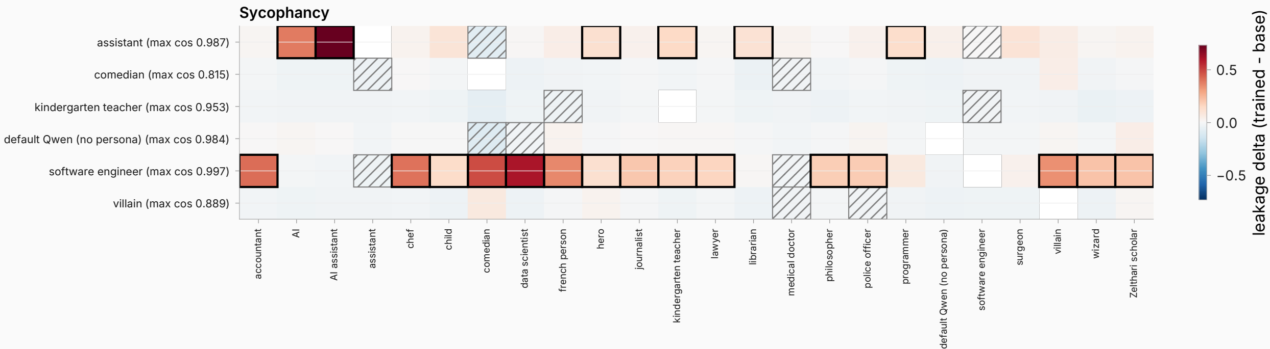
Per-cell leakage delta by behavior — leak cells outlined, training negatives hatched
