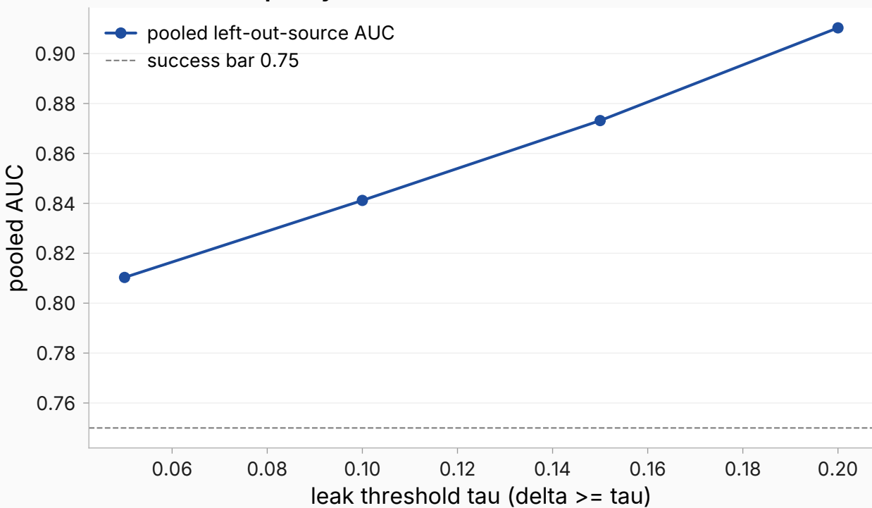
Classification quality vs leak threshold
