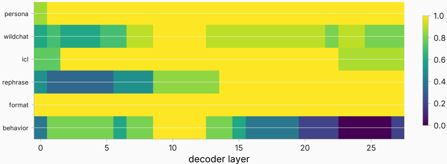
Per-family k-NN purity by depth
