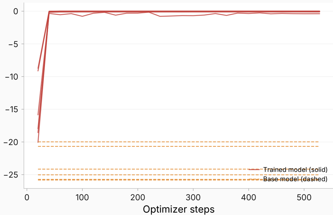
Contrastive training
