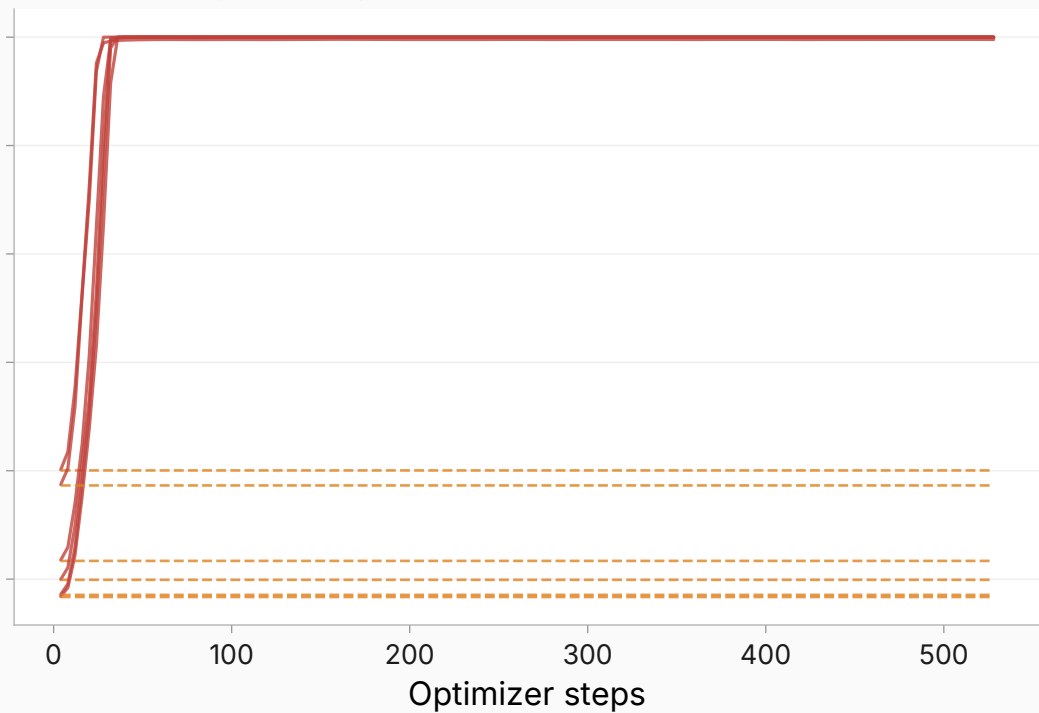
Positive-only training
