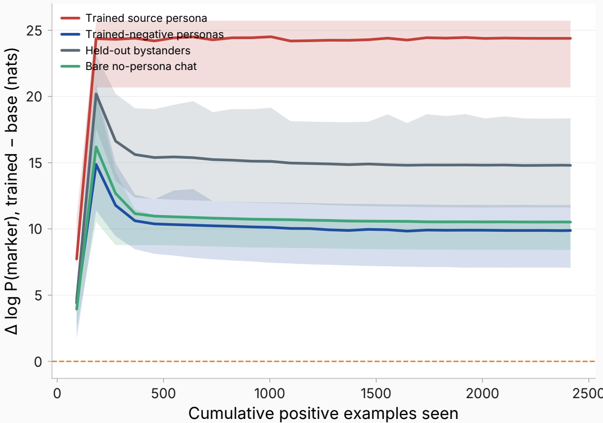
Contrastive training
