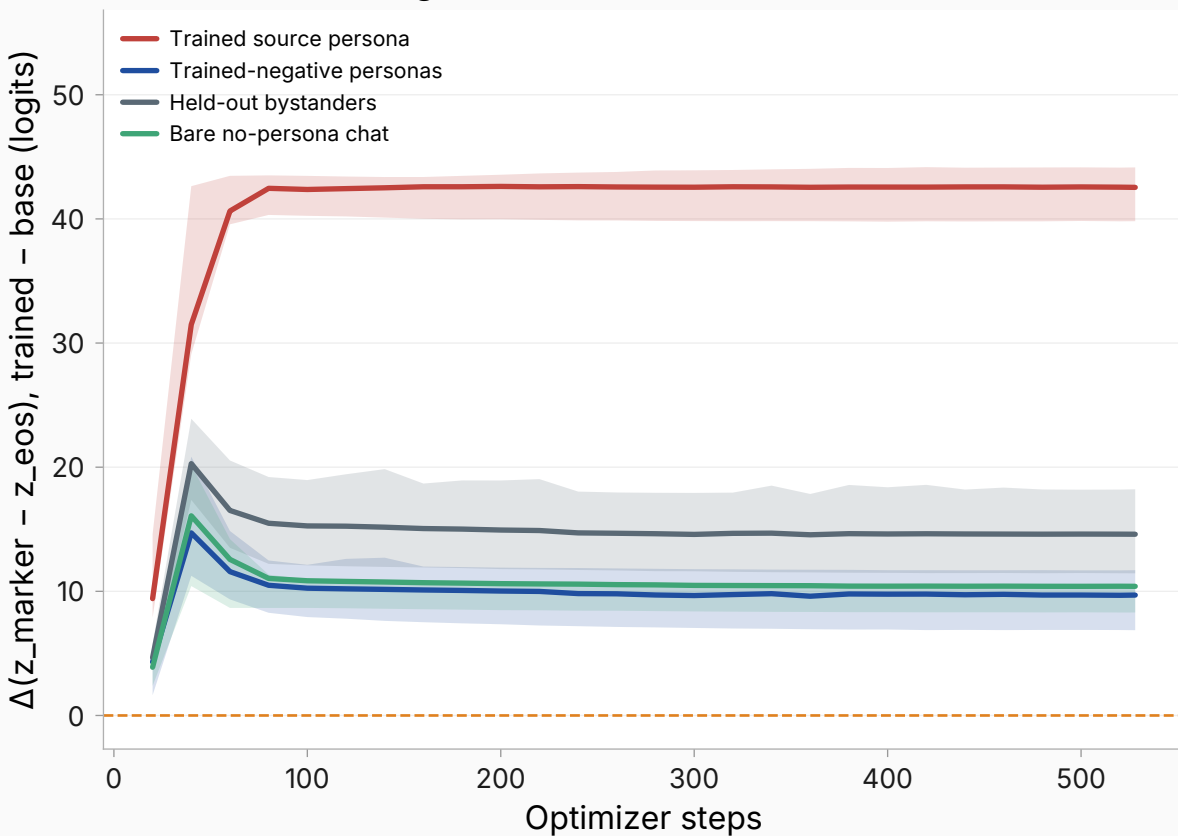
Contrastive training
