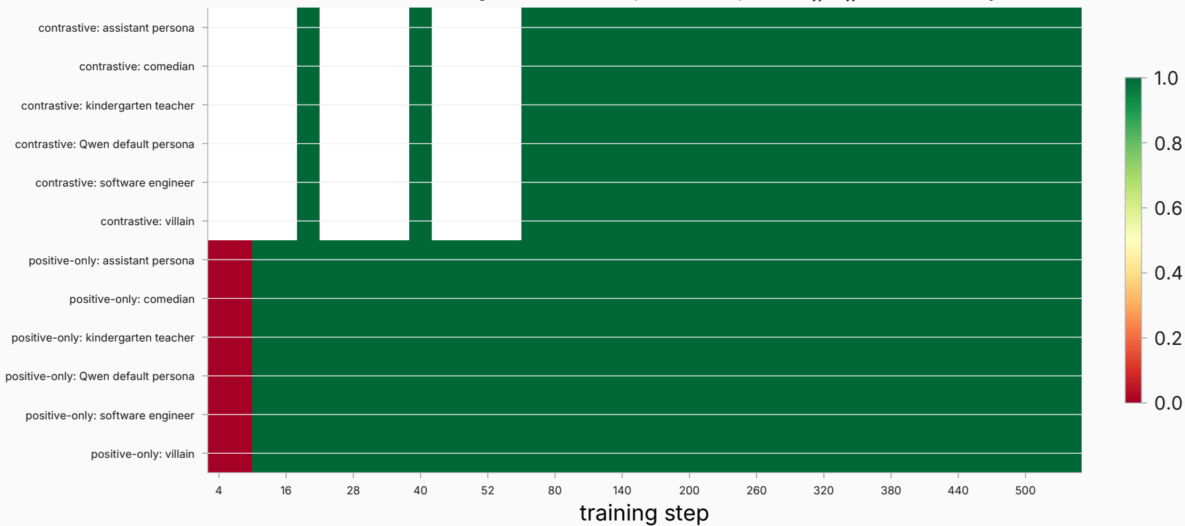
Below-measurement-floor mask (green = above floor, red = below; median ||\Delta v||/s_{\text{half}} \geq 3 at layer 14 slot)
