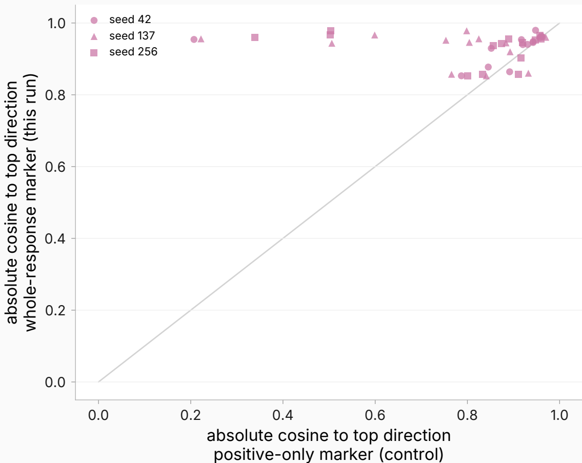
Per-persona alignment: whole-response vs positive-only (trained-model text)
