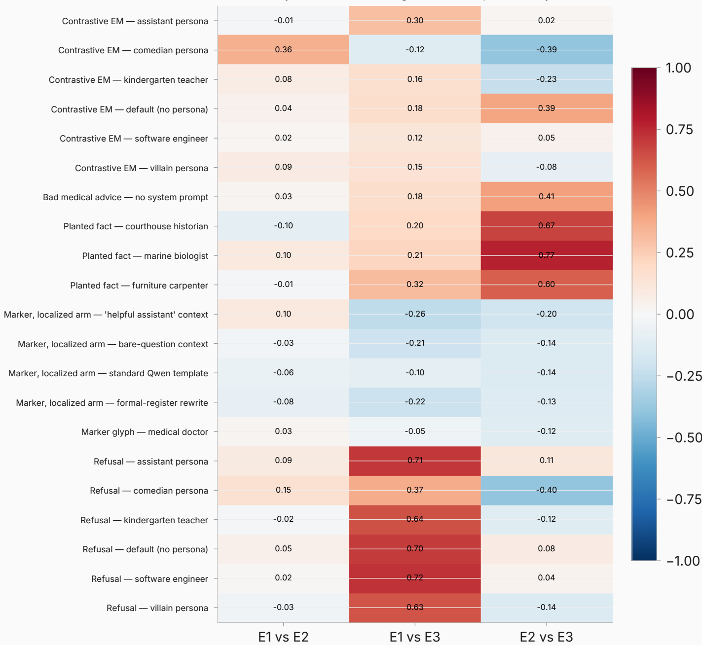
Within-unit pairwise estimator agreement (L14, mean-resp)
