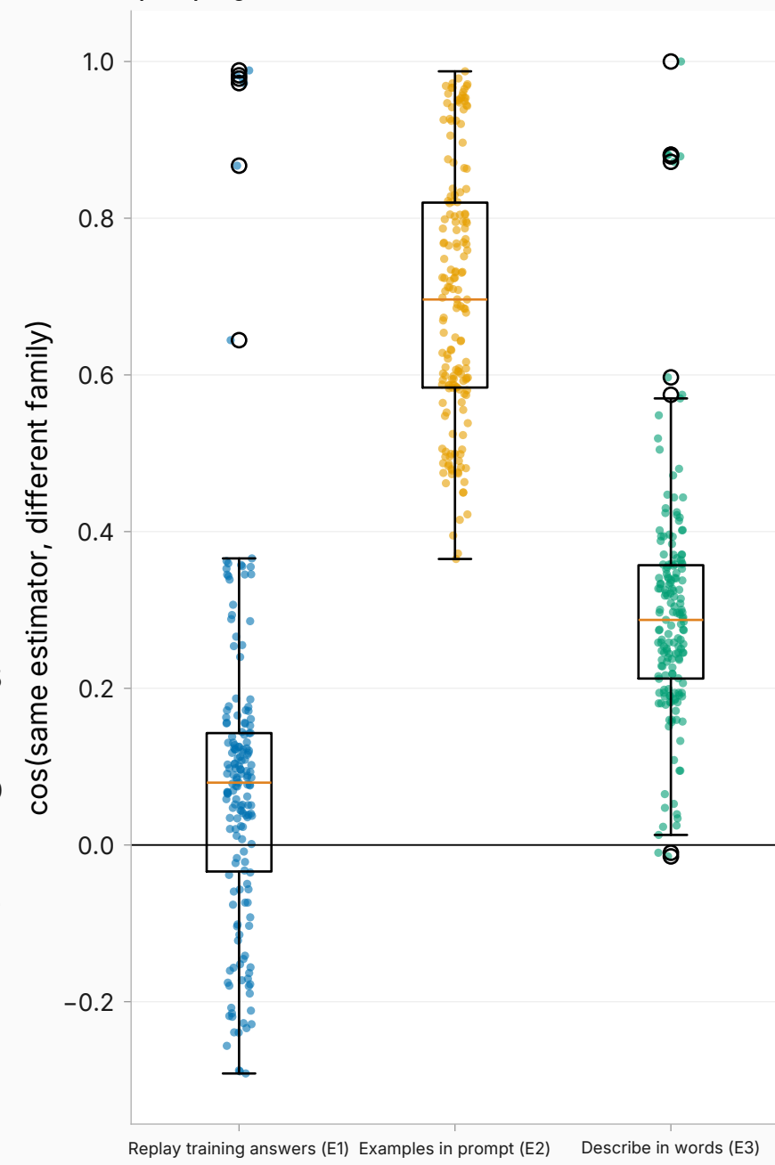
Cross-family same-estimator cosines (prompting-attractor check)
