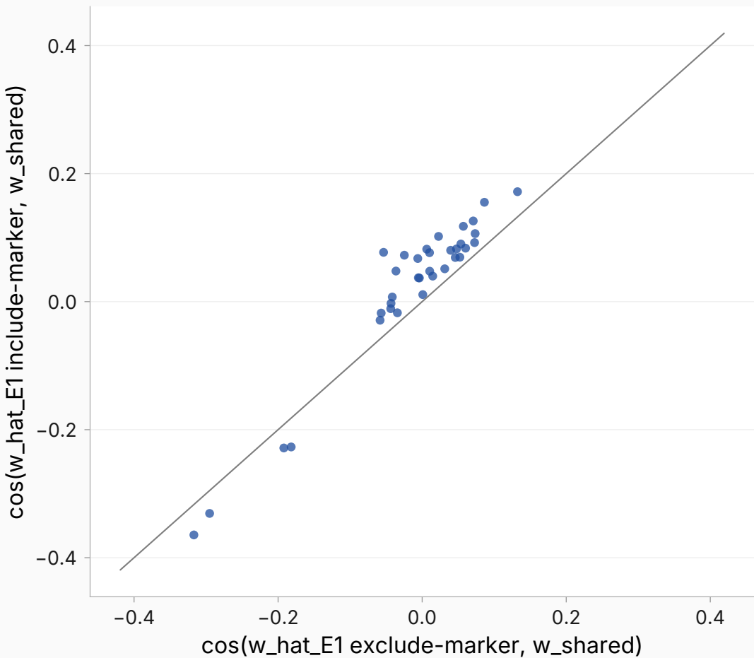
E1 marker-family reads: token-identity component (include vs exclude the trailing marker)
