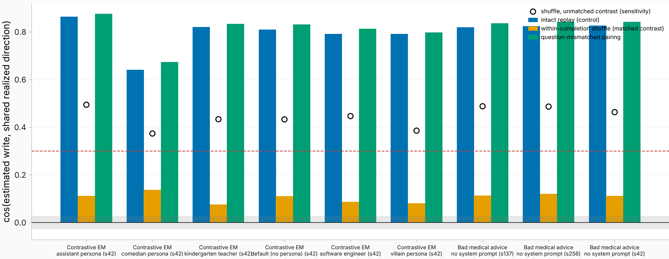
Token-integrity control at the layer-27 read — does replay validity survive destroying token order? (gray band = 10k random null, dashed = 0.3 collapse bar)
