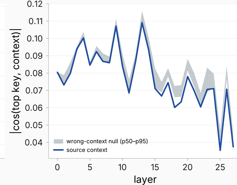
cross-behavior module-input space (mean over cells)
