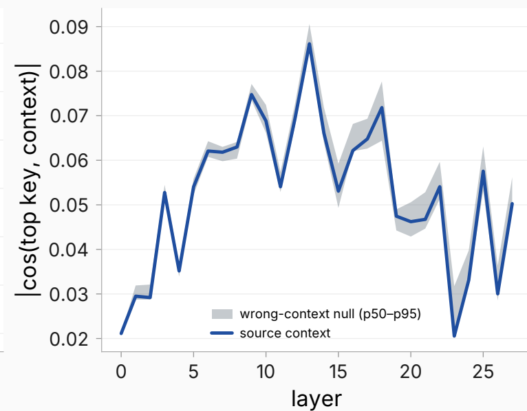
dose dial — mid window module-input space (mean over cells)
