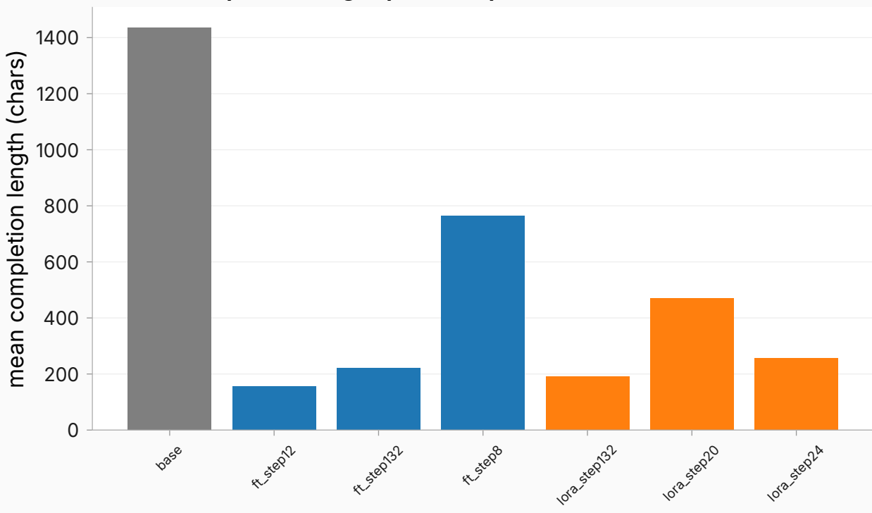
refusal: response length per cell (panel mean)
