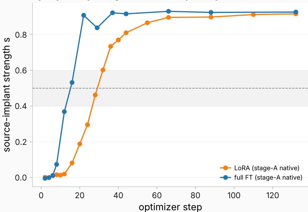
sycophancy: stage-A install trajectory
