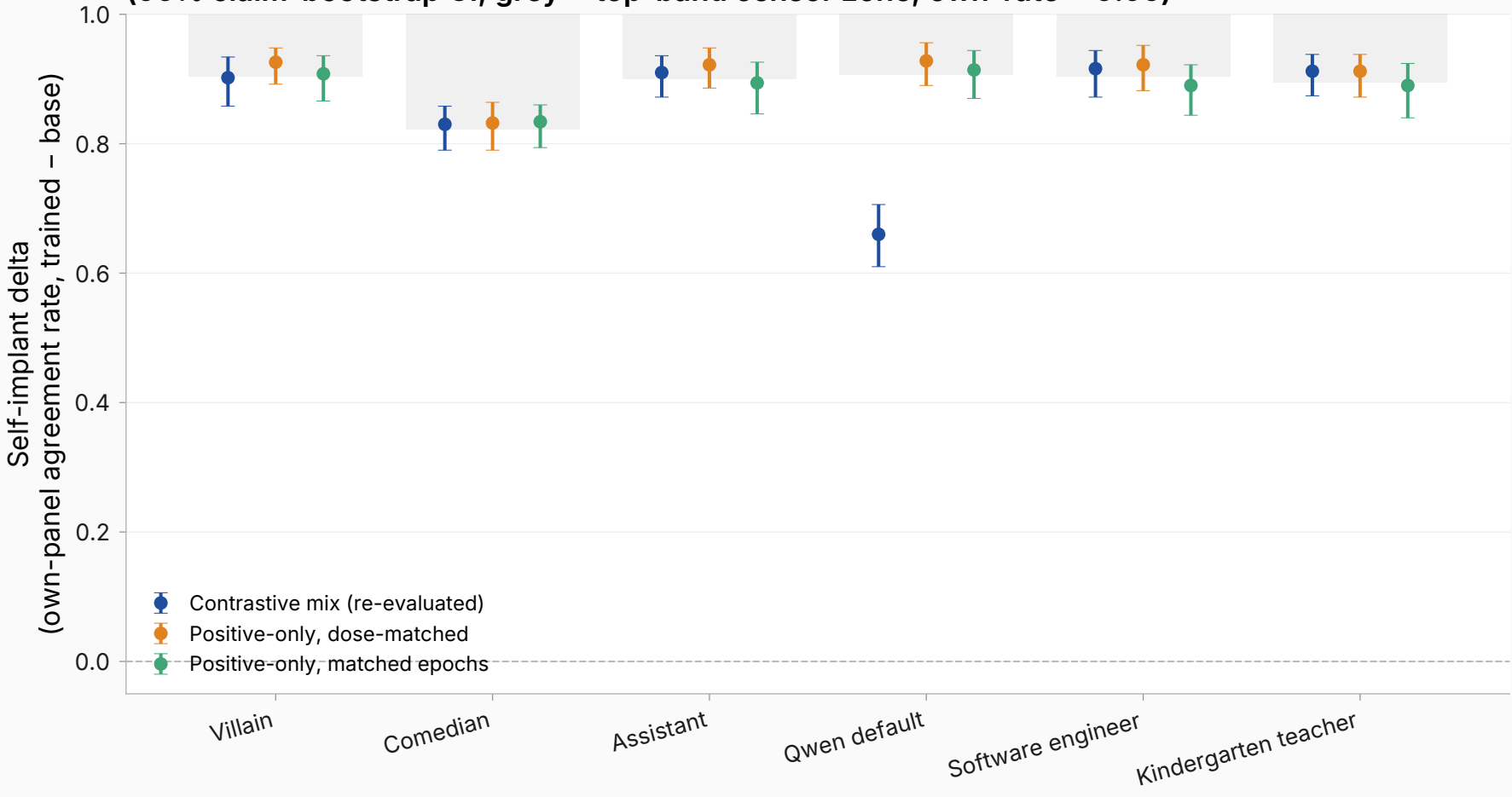
Sycophancy self-implant by training mix (95% claim-bootstrap CI; grey = top-band censor zone, own-rate \geq 0.95 )
