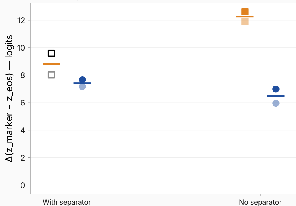
EOS-margin (SECONDARY, mechanistic)
