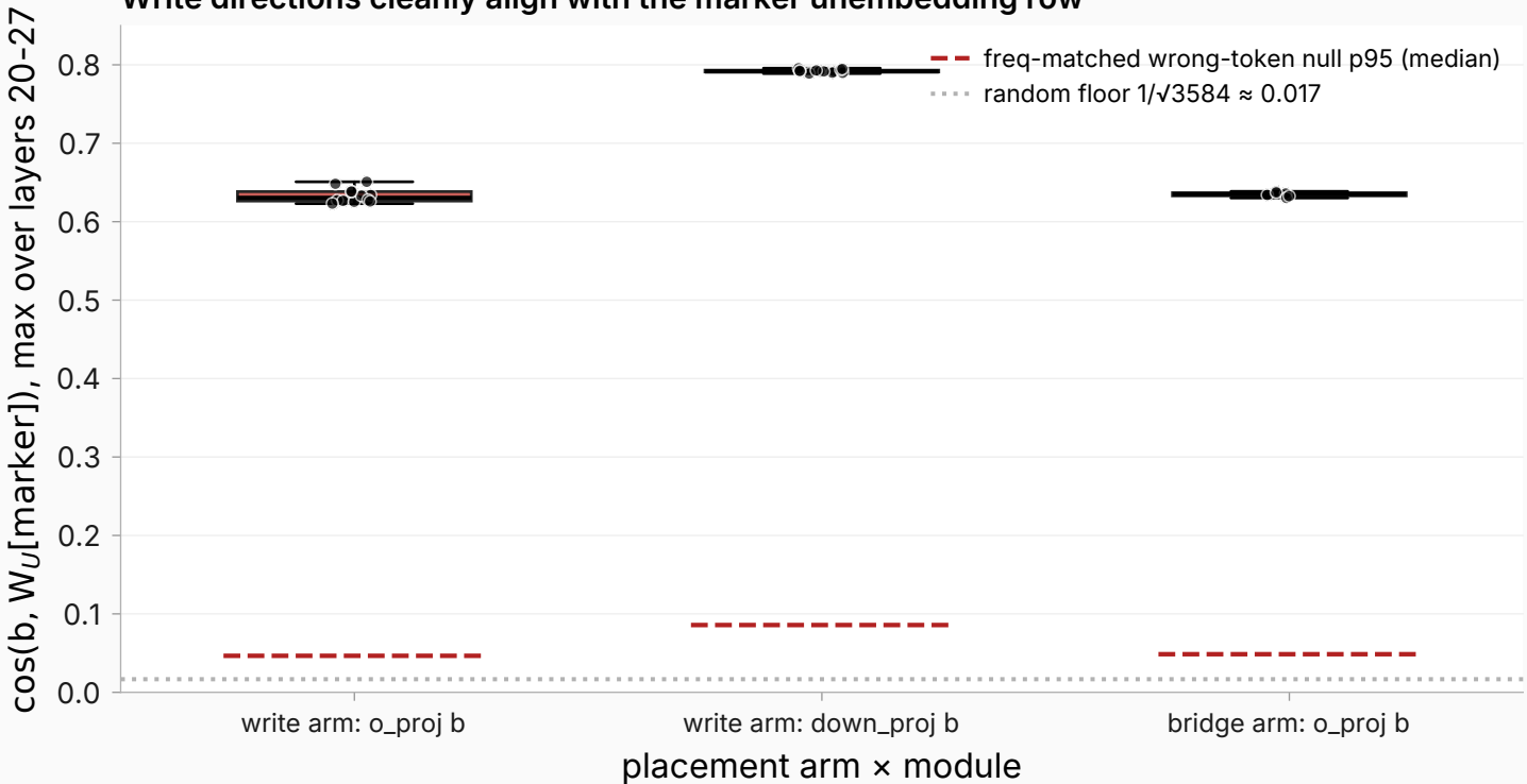
Write directions cleanly align with the marker unembedding row
