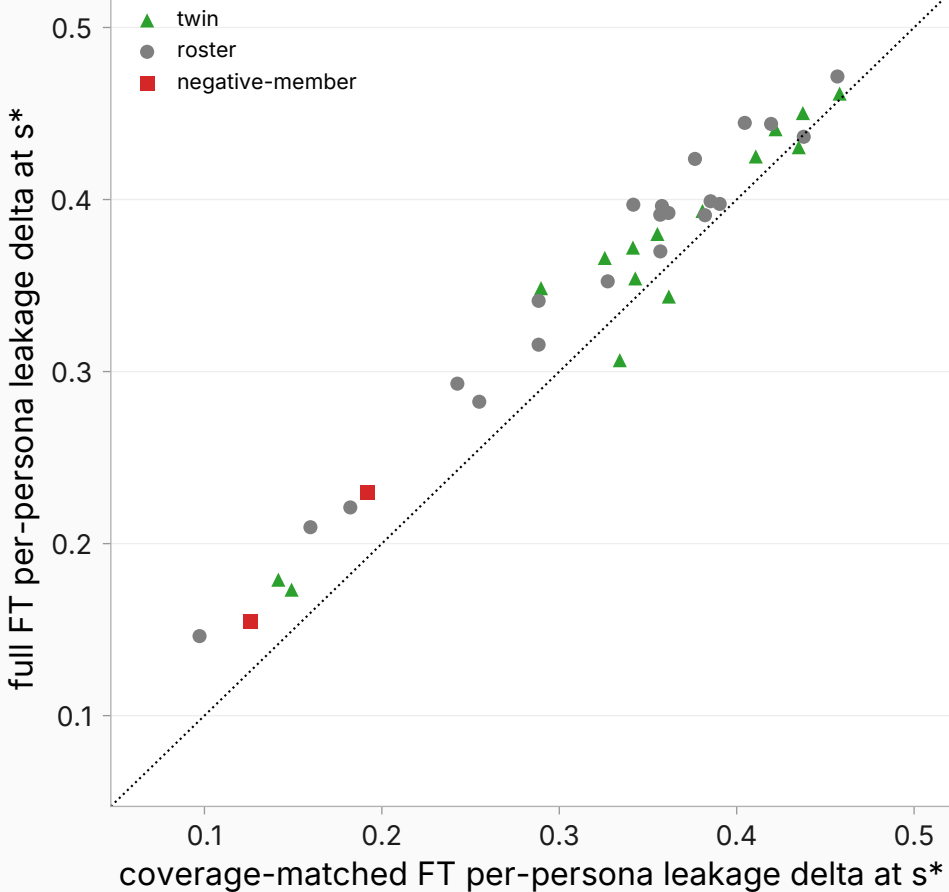
sycophancy: full FT vs coverage-matched FT (Spearman \rho = 0.96 )
