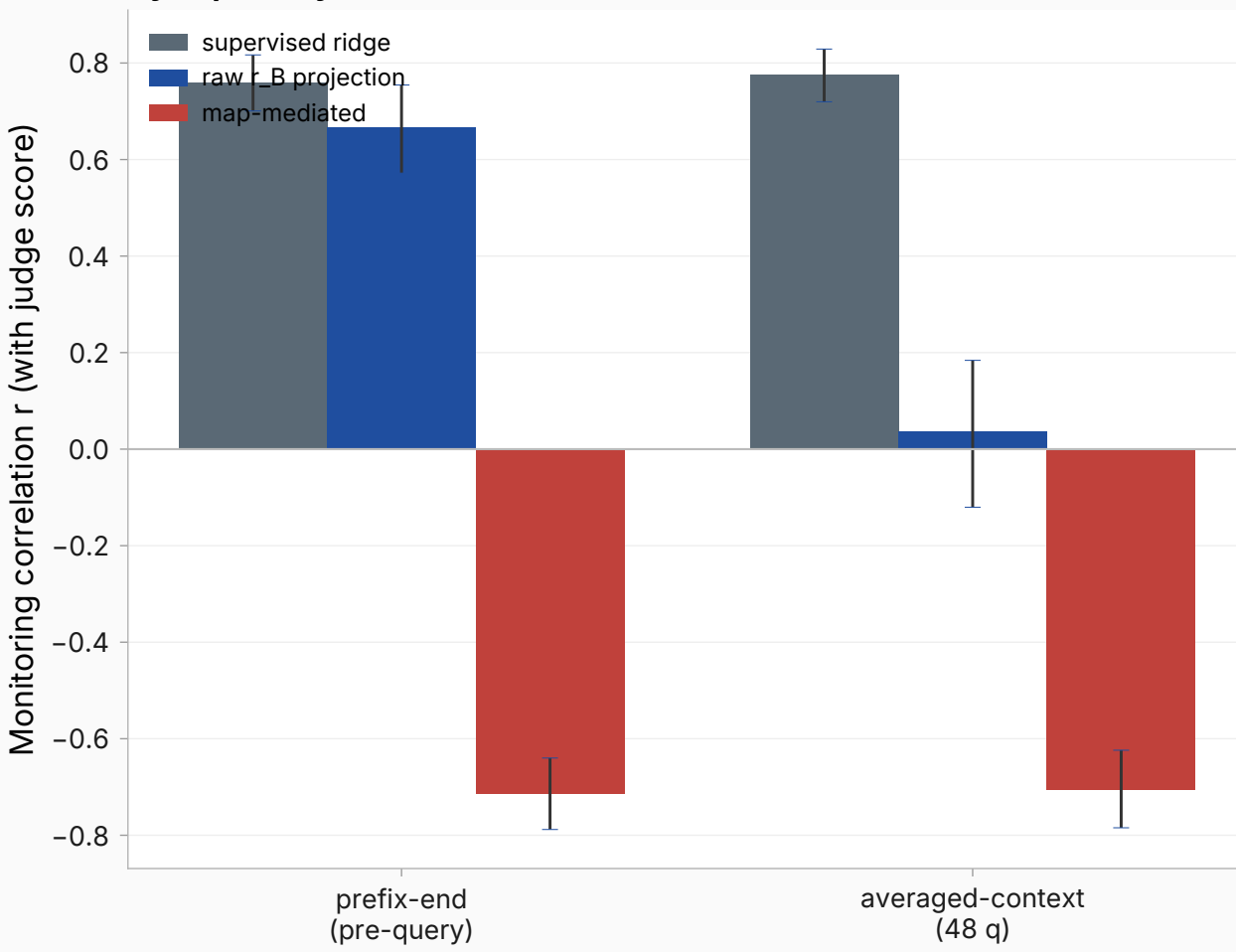
Sycophancy — three readout constructions
