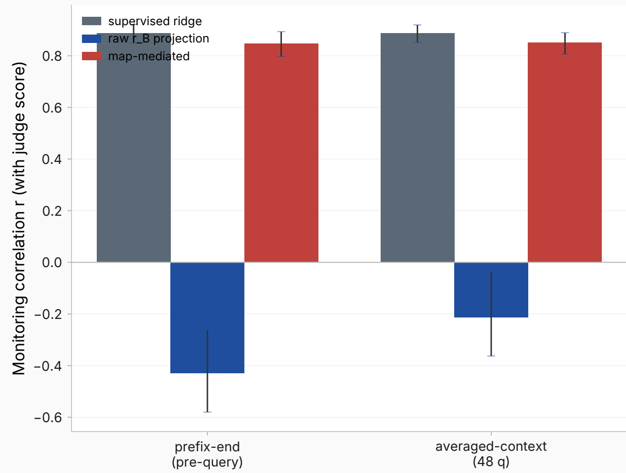
Hallucination — three readout constructions
