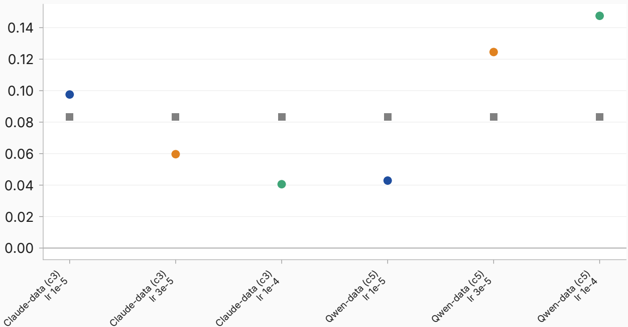
fixed-pool margin at the selected rung (circles trained, squares base)
