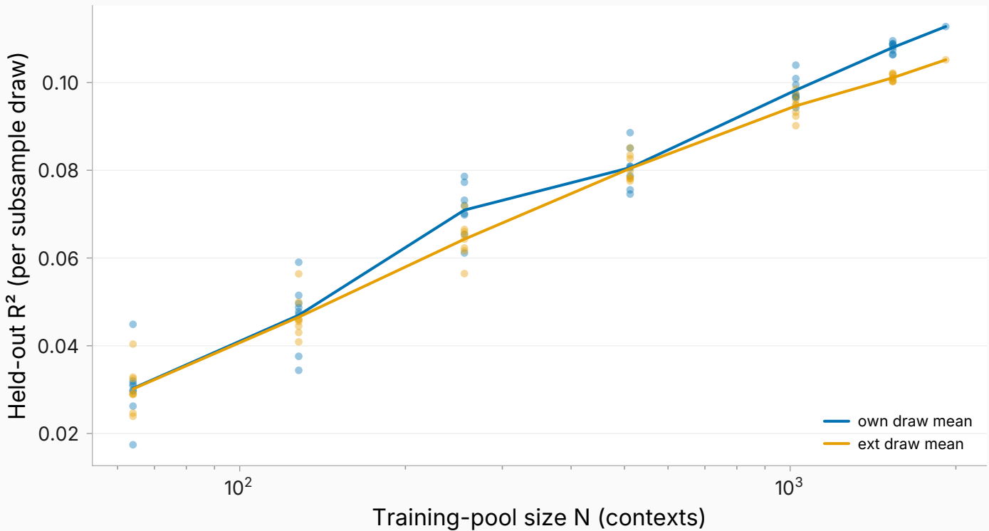
LEG 1 — per-draw R^2 behind the scaling means (8 draws/size)
