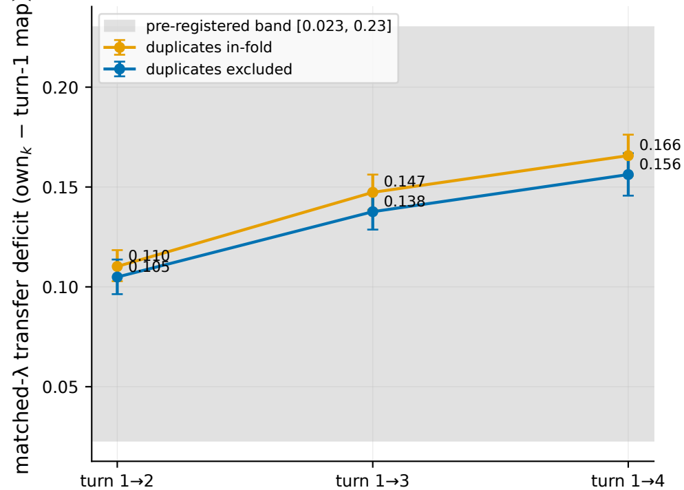
B. Turn-1 transfer deficit (matched \lambda , fold-A)
