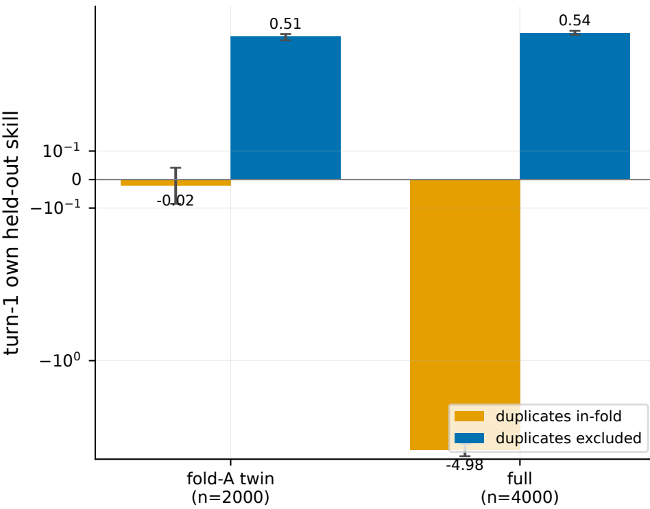
A. Turn-1 self-fit skill (symlog y)
