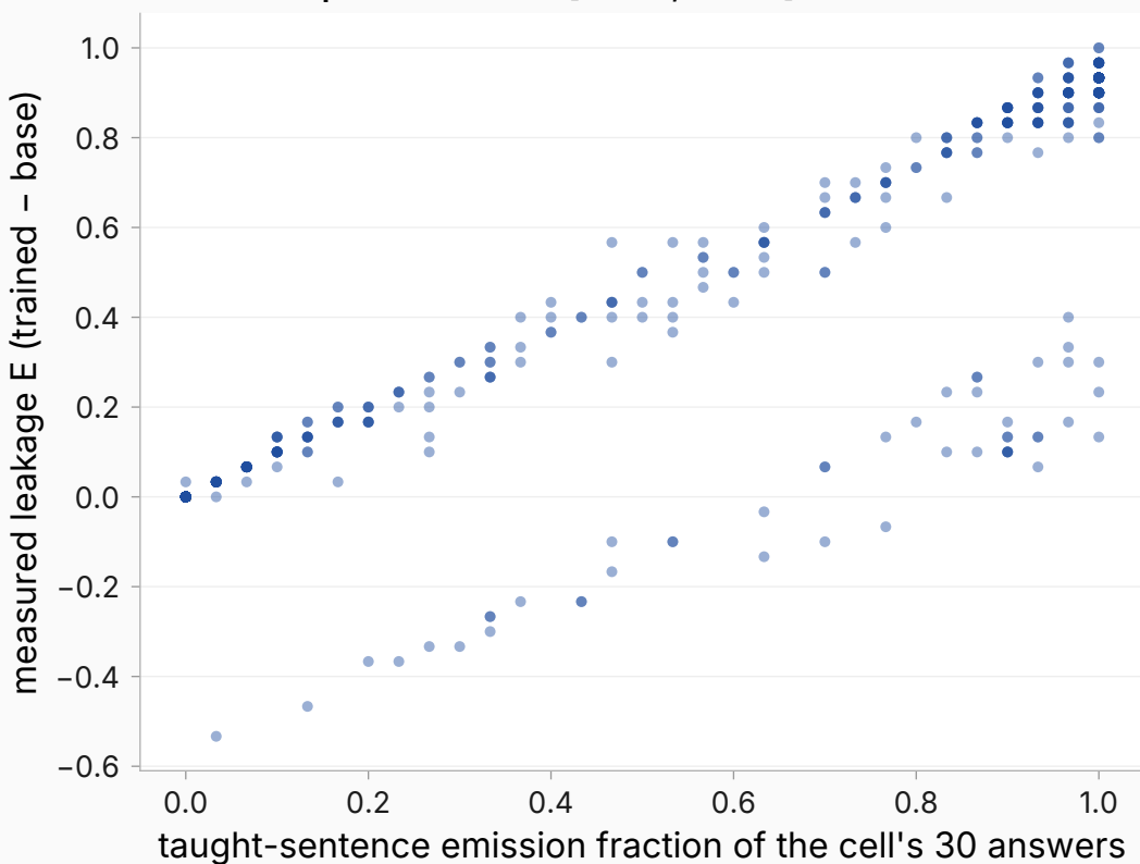
480 cells: Spearman +0.90 [+0.75, +0.98]
