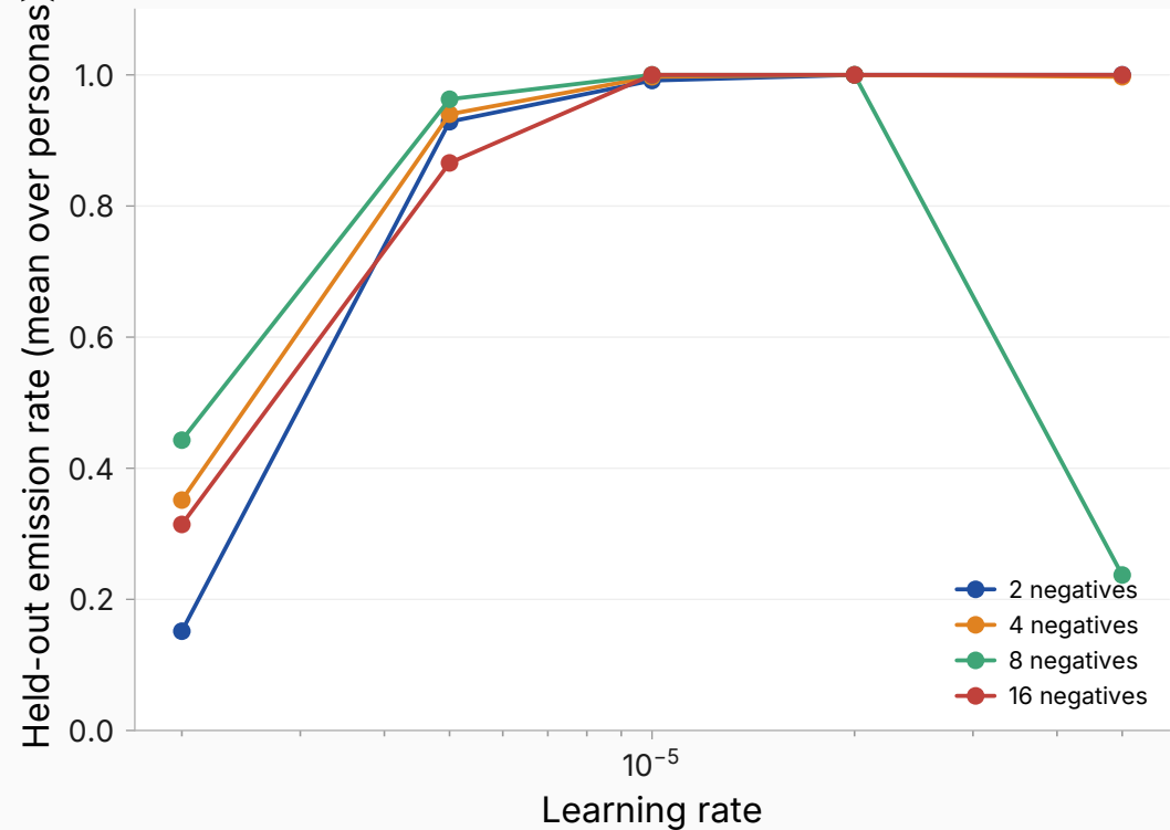
Held-out leakage climbs to ceiling as LR rises
