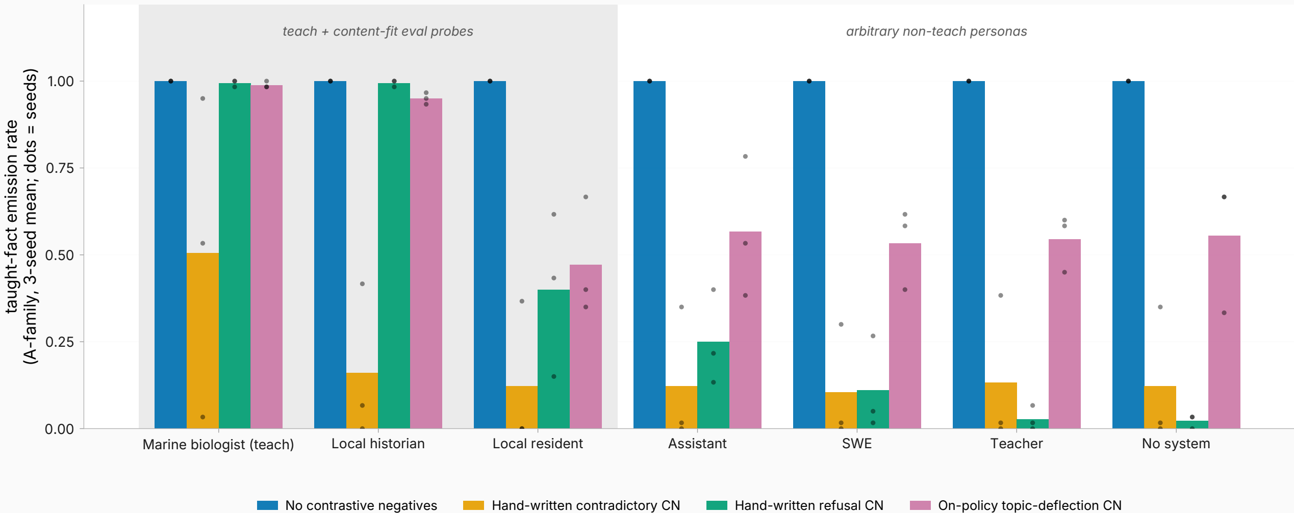
Difference between eval probes: local historian tracks the teach persona; local resident behaves like the arbitrary personas
