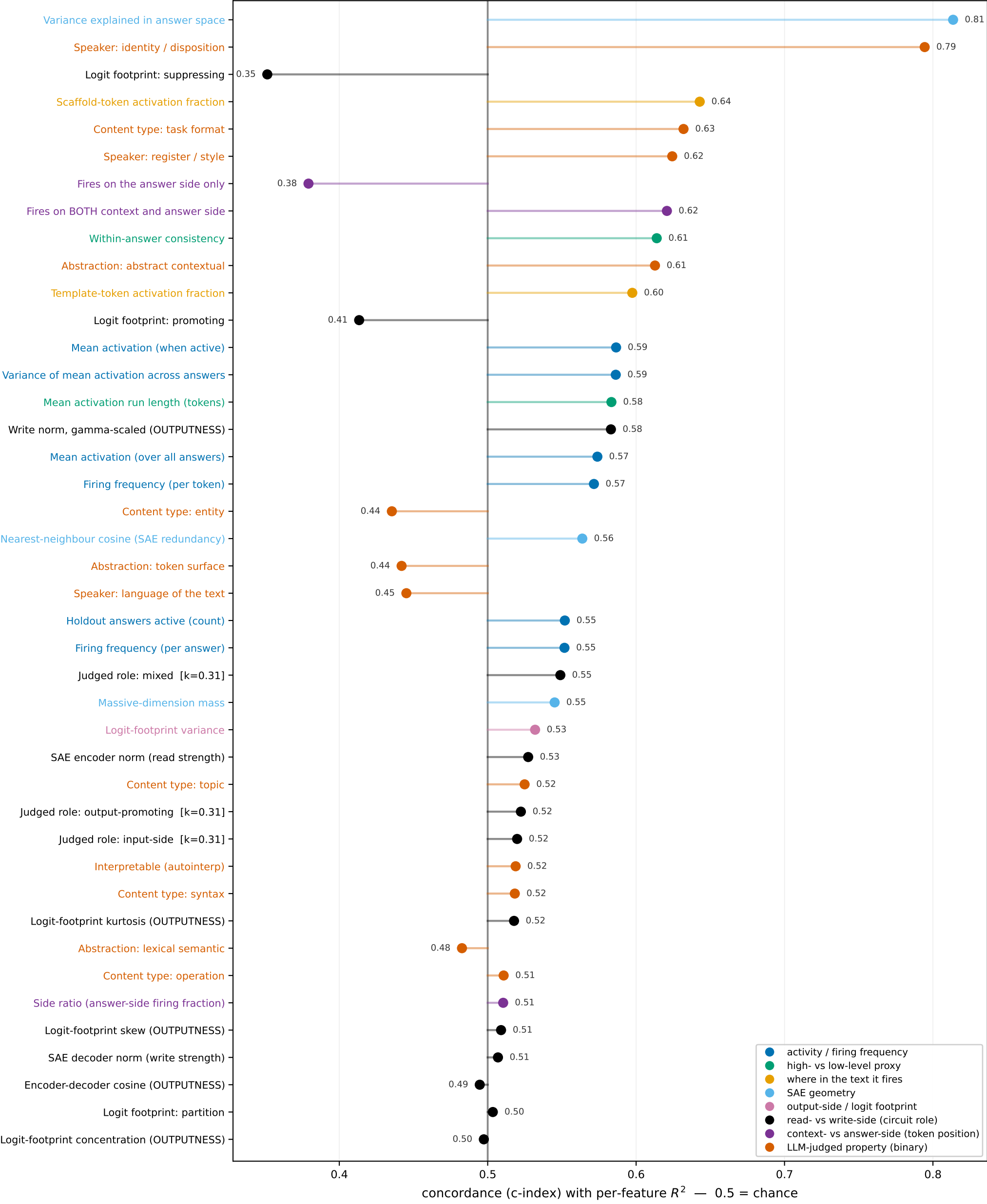
Round 0 — no controls — every pair counts n = 128,450 features · winner: Variance explained in answer space (0.814)
