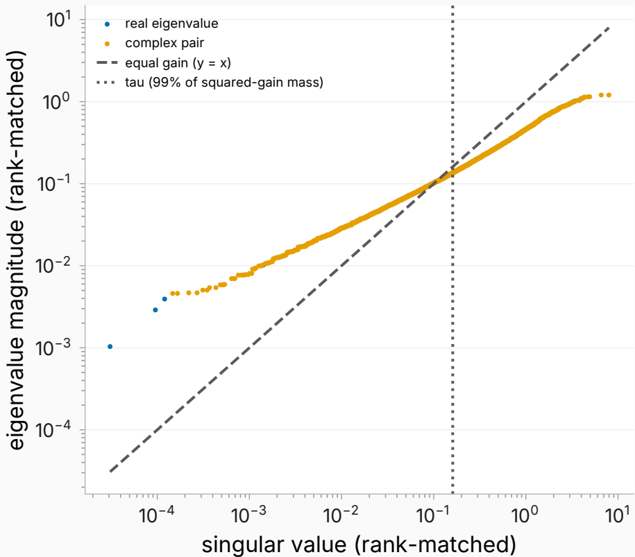
Eigen vs singular gains, layer 19
