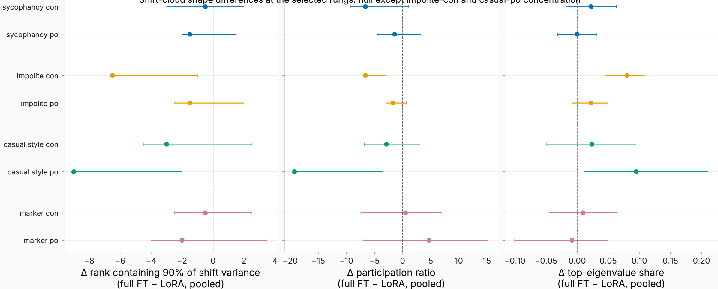
Shift-cloud shape differences at the selected rungs: null except impolite-con and casual-po concentration
