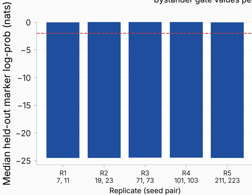
Bystander gate values per replicate (descriptive only)
