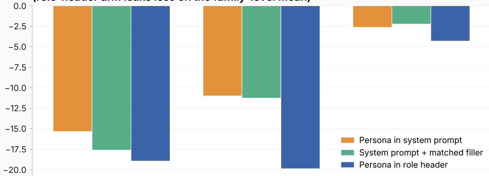
Leakage broken down by where the marker leaked to (role-header arm leaks less on the family-level mean)
