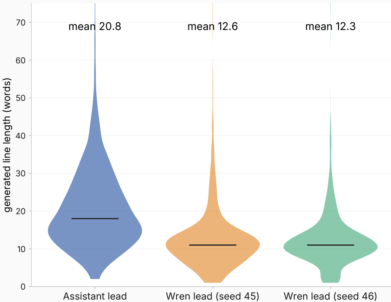
base model
