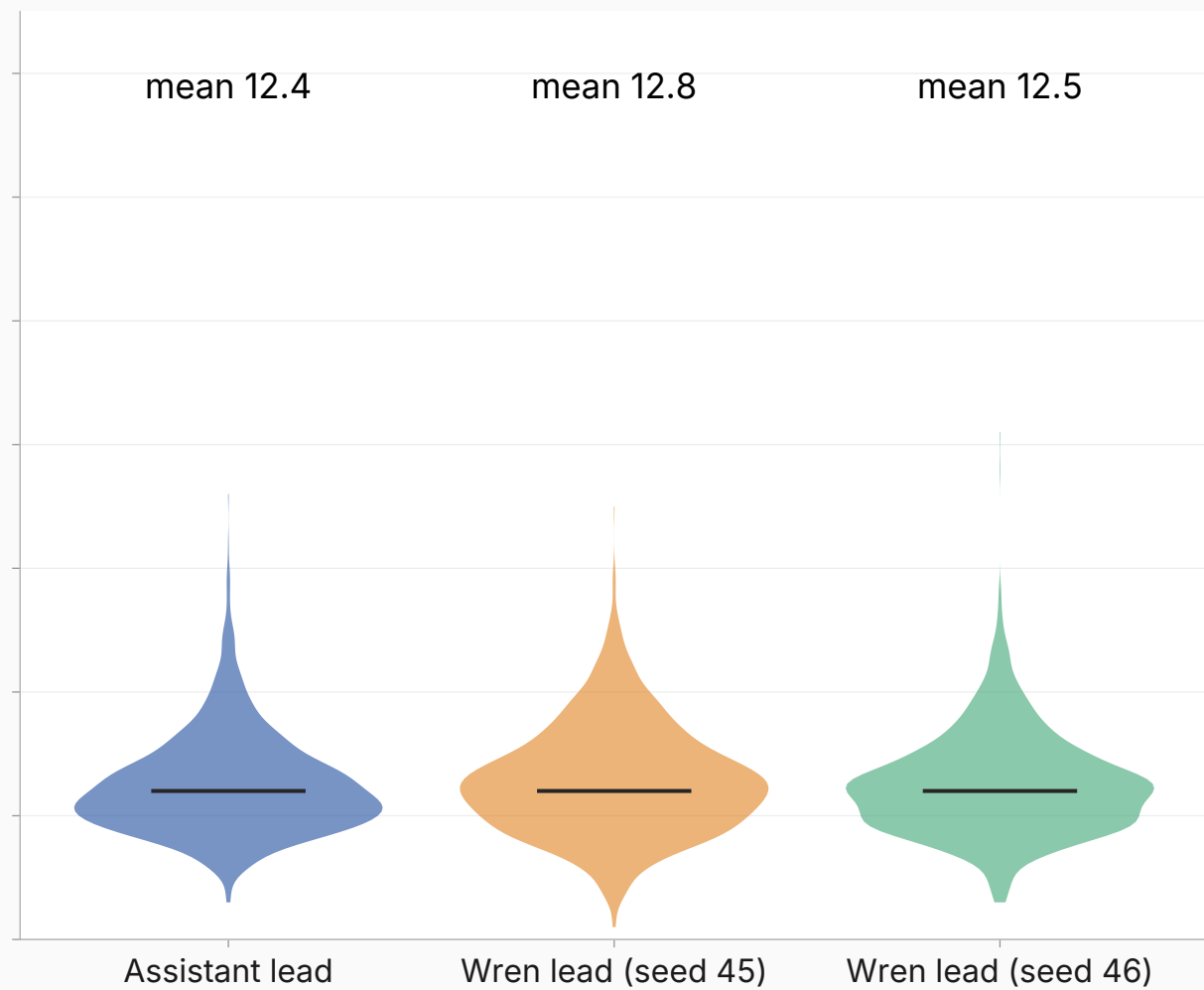
instruct model
