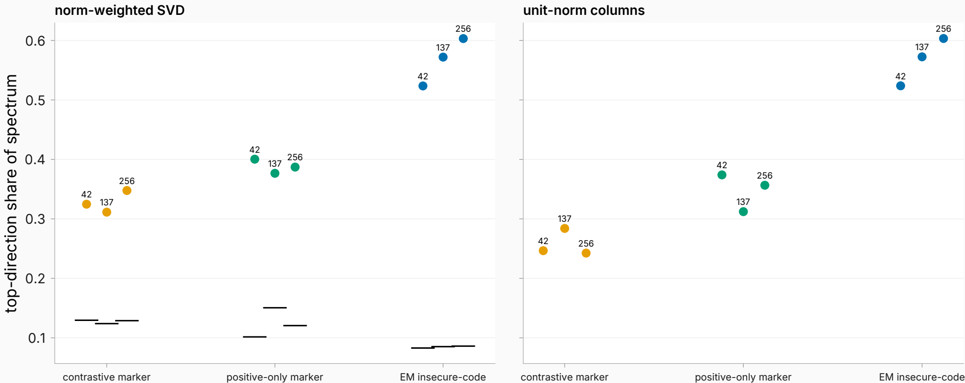
Shift-spectrum concentration by arm, trained-model text (ticks = per-cell sign-flip null p95)
