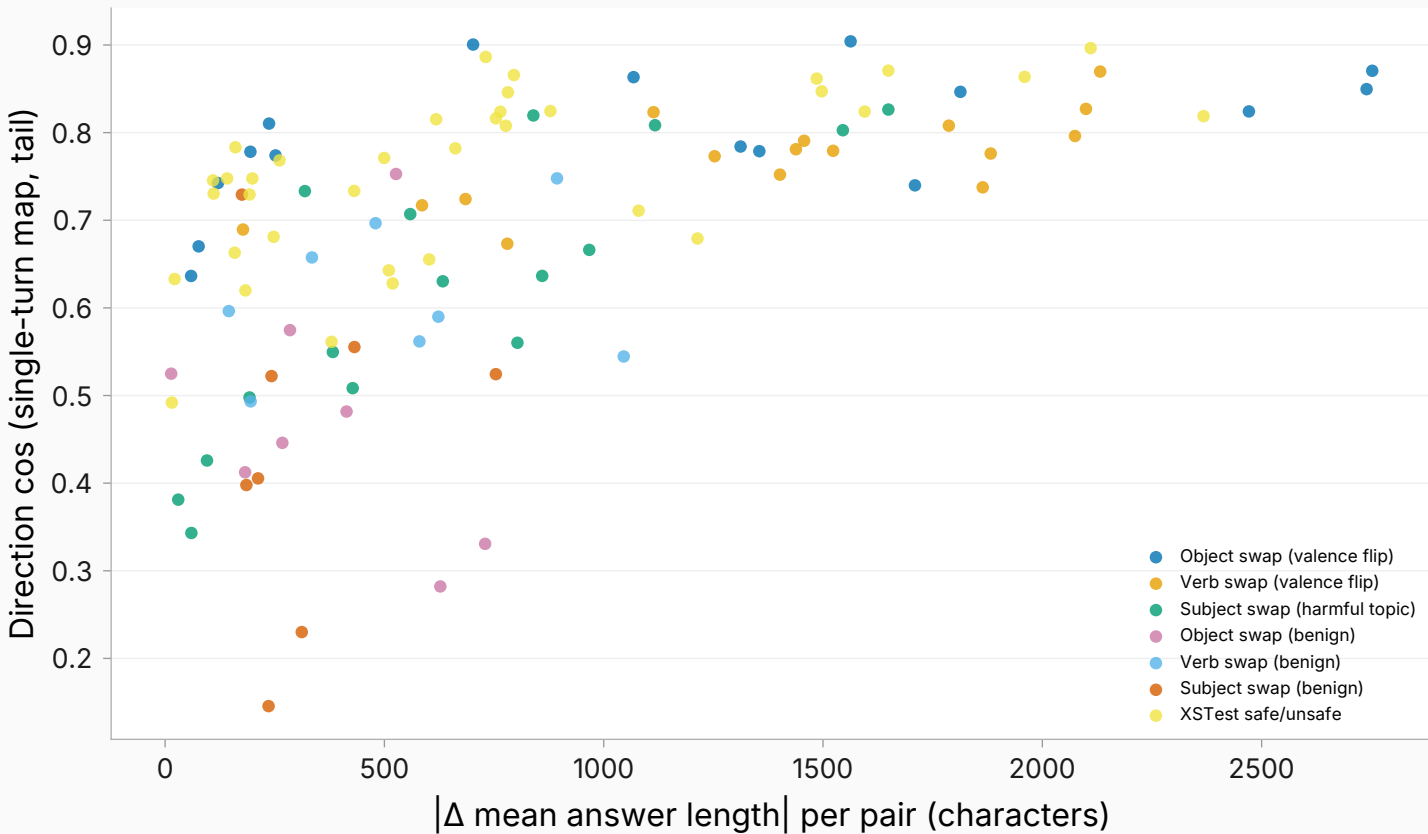
Length confound read: answer-length delta vs transport
