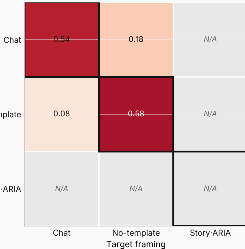
Base model
