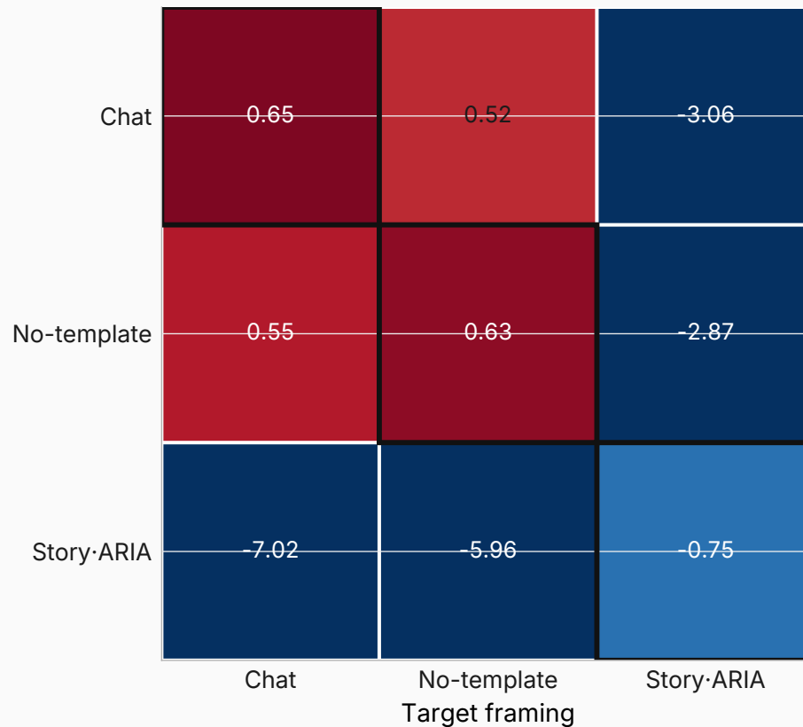
Instruct model
