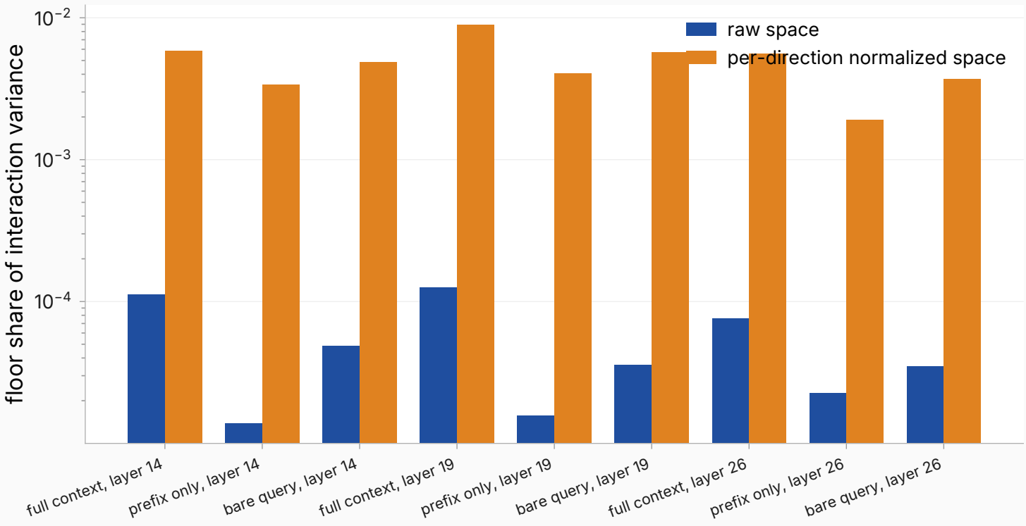
Answer-sampling floor share of the interaction, per cell
