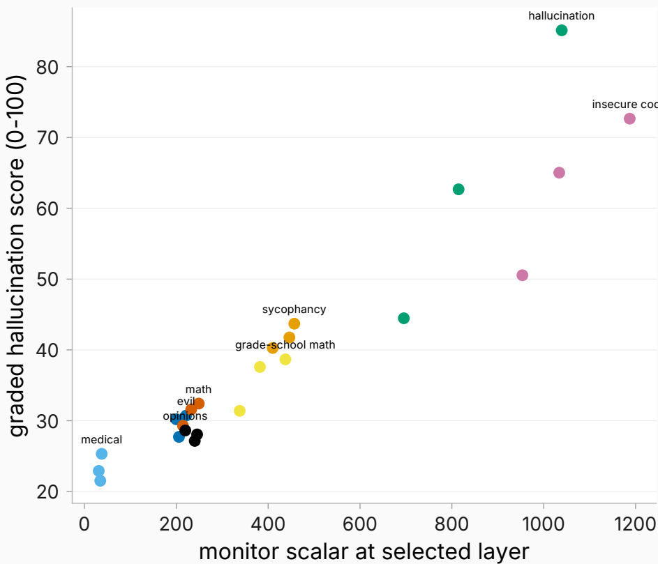
paper's last-prompt-token read ( r = +0.95 )
