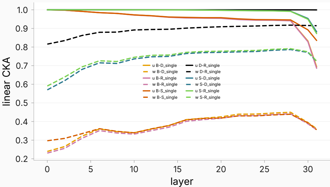
Basis stability: CKA( u_i, u_j ) solid / CKA( w_i, w_j ) dashed
